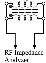
Measuring Circuit :
