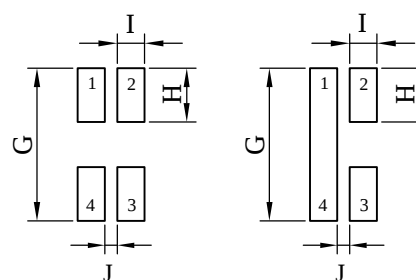
Dual Inductor Mode Series Mode (PCB Pattern)
