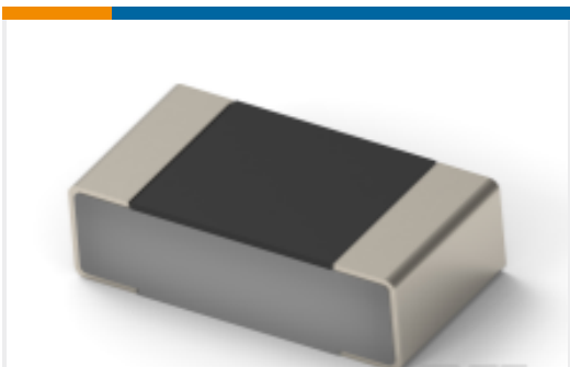
TE Part #2176467-5 TLRP 1206 1.0W R020 1% 50PPM 5K RL
