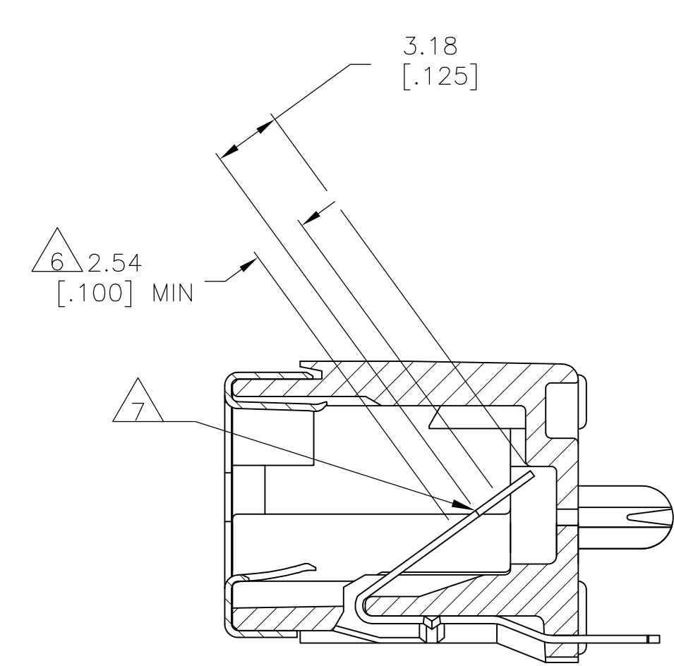
SECTION J-J
