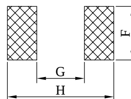
( PCB Pattern )
